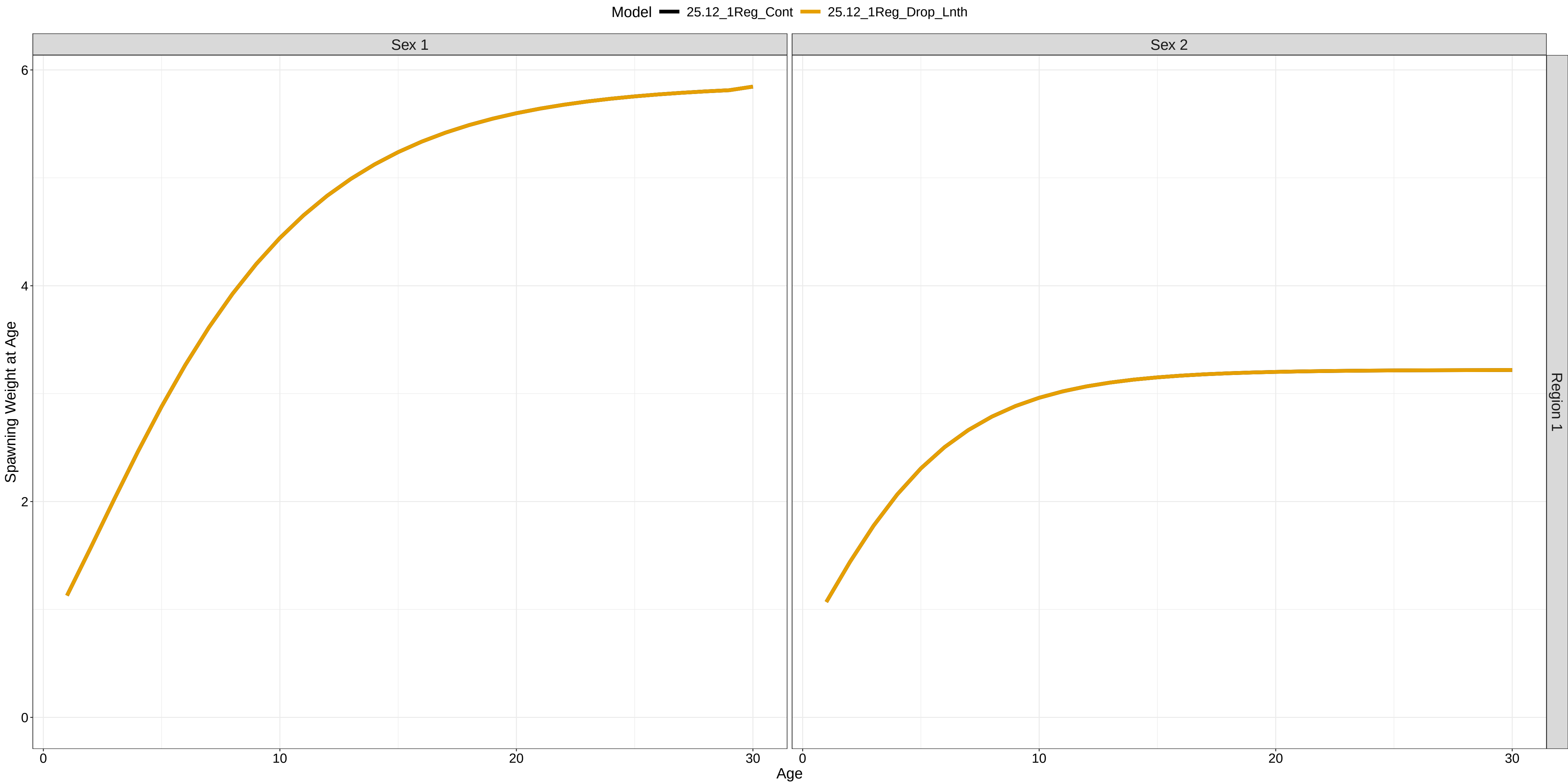
Weight-at-Age
